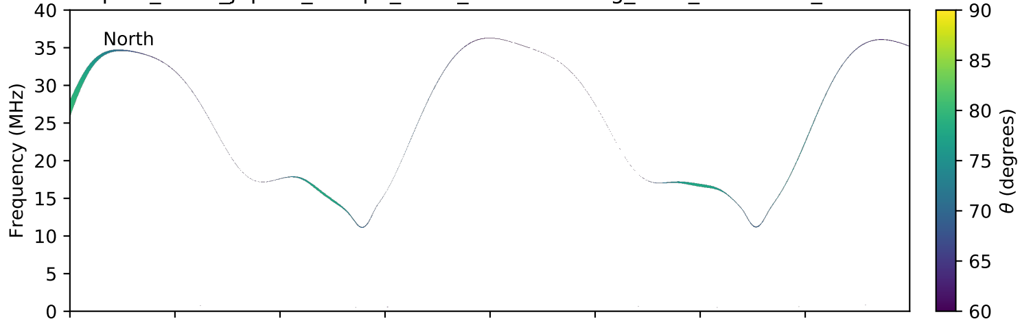
expres_earth_jupiter_europa_isaac_lossc-wid1deg_3kev_20160201_v01.cdf
