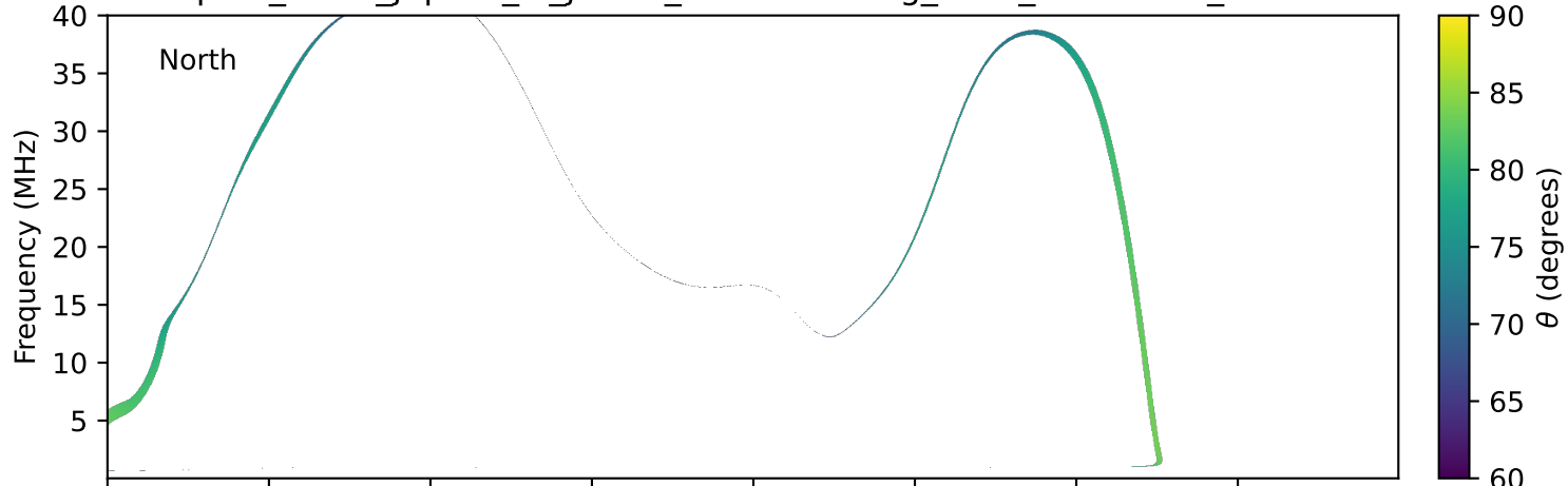
expres_earth_jupiter_io_jrm33_lossc-wid1deg_3kev_20151212_v11.cdf
