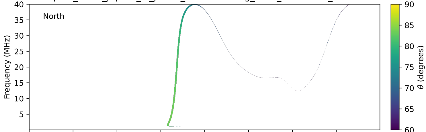
expres_earth_jupiter_io_jrm33_lossc-wid1deg_3kev_20151201_v11.cdf
