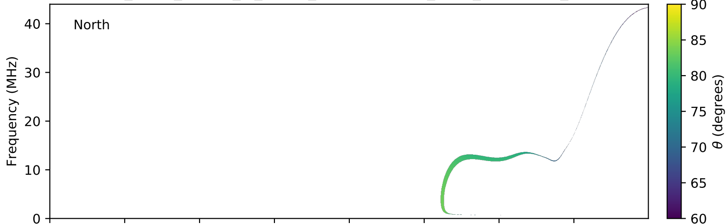
expres_earth_jupiter_io_jrm09_lossc-wid1deg_3kev_20151229_v01.cdf
