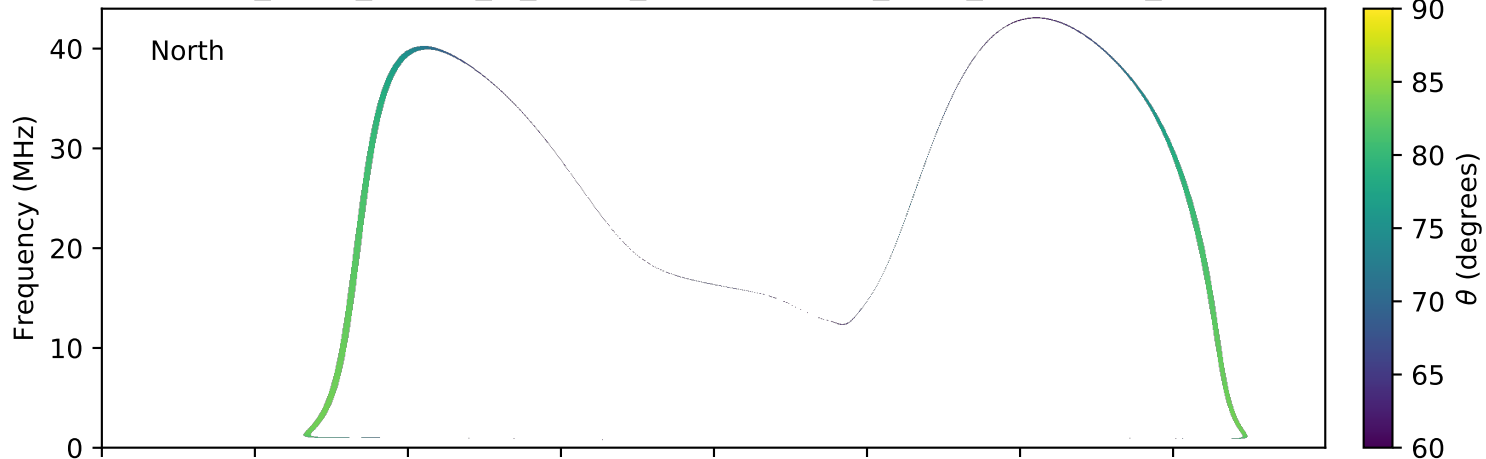
expres_earth_jupiter_io_jrm09_lossc-wid1deg_3kev_20151226_v01.cdf
