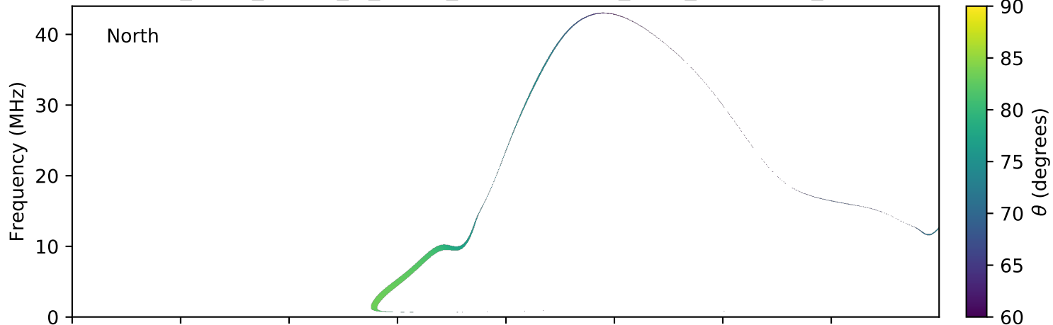
expres_earth_jupiter_io_jrm09_lossc-wid1deg_3kev_20151224_v01.cdf
