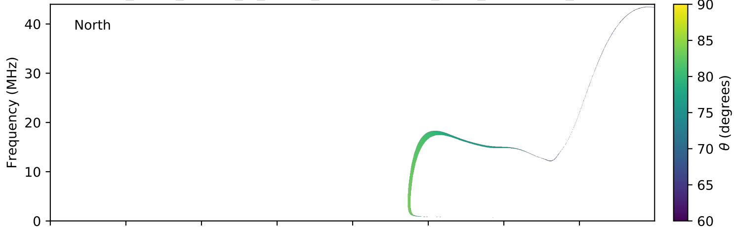
expres_earth_jupiter_io_jrm09_lossc-wid1deg_3kev_20151222_v01.cdf
