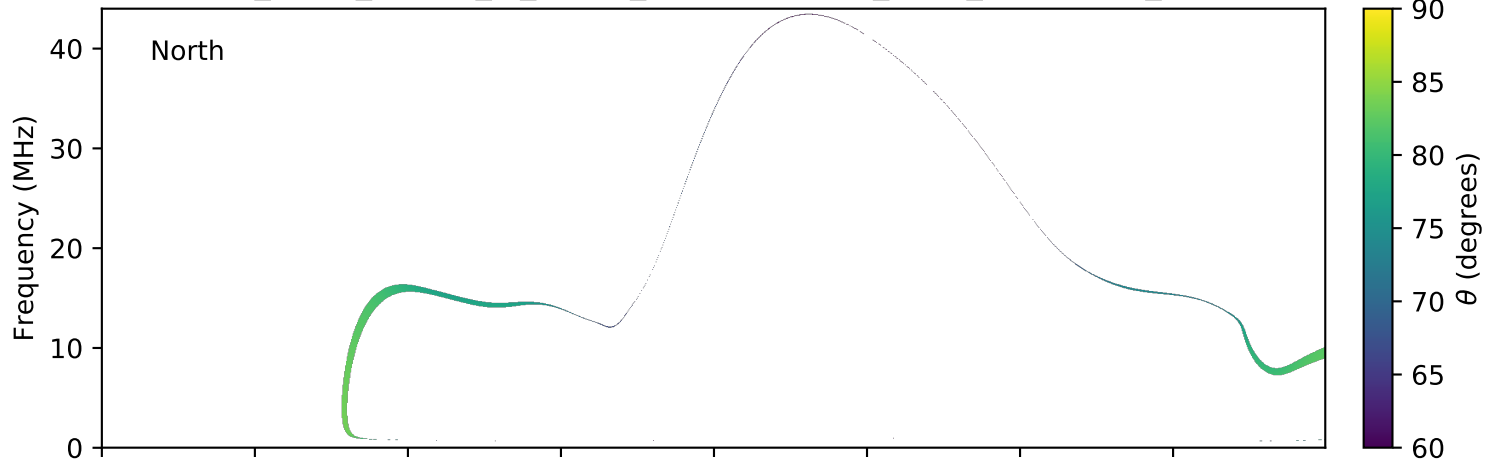
expres_earth_jupiter_io_jrm09_lossc-wid1deg_3kev_20151210_v01.cdf
