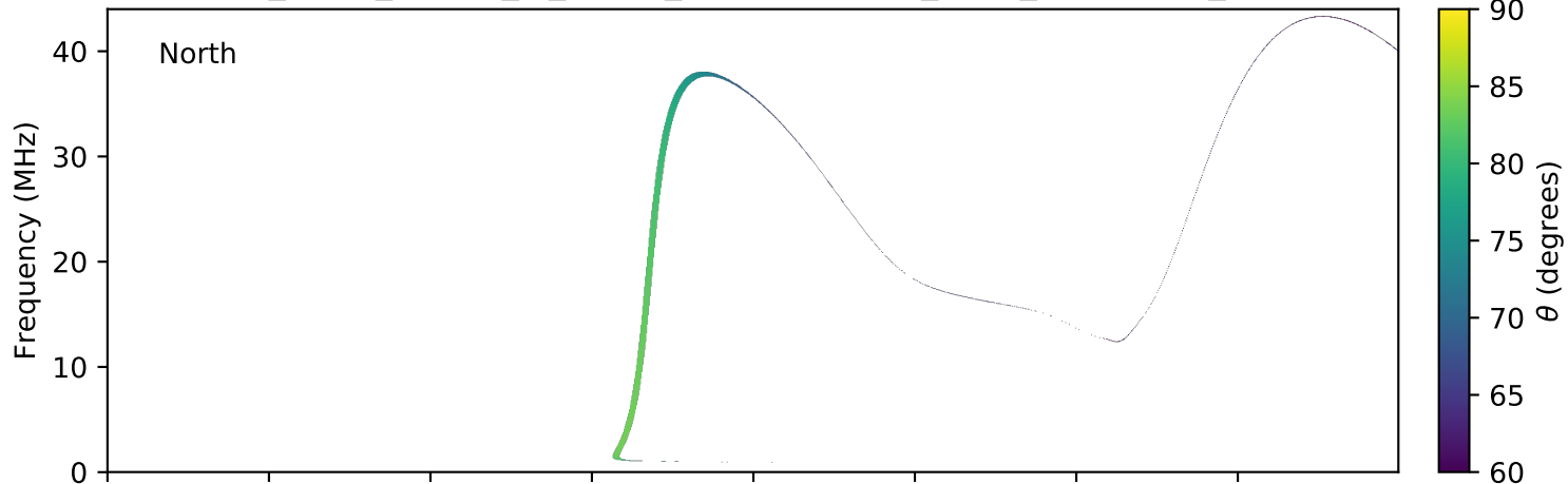
expres_earth_jupiter_io_jrm09_lossc-wid1deg_3kev_20151201_v01.cdf
