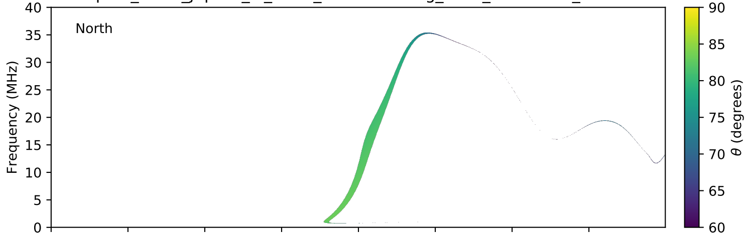
expres_earth_jupiter_io_isaac_lossc-wid1deg_3kev_20151231_v01.cdf
