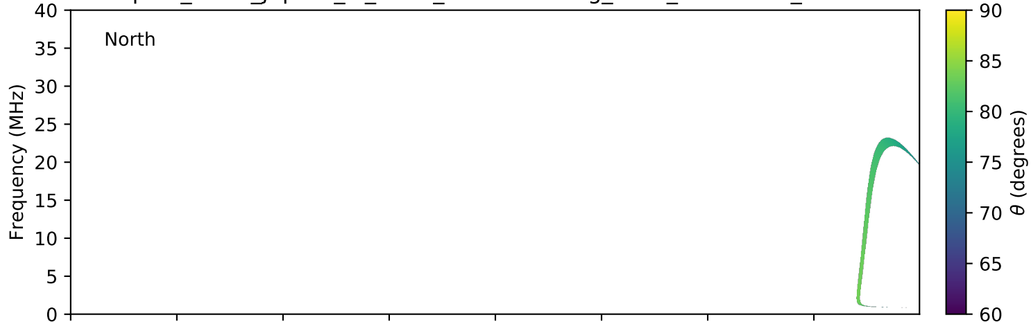
expres_earth_jupiter_io_isaac_lossc-wid1deg_3kev_20151227_v01.cdf
