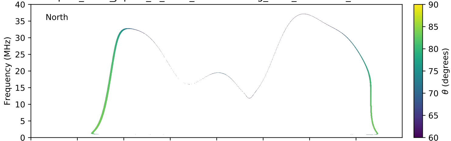
expres_earth_jupiter_io_isaac_lossc-wid1deg_3kev_20151226_v01.cdf
