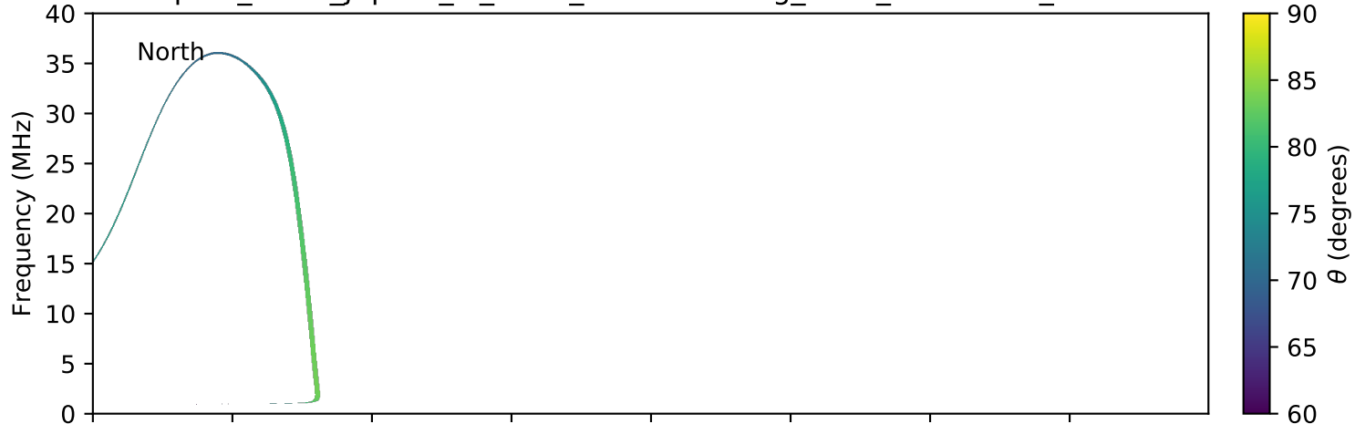
expres_earth_jupiter_io_isaac_lossc-wid1deg_3kev_20151225_v01.cdf
