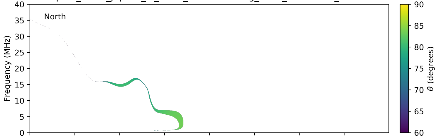
expres_earth_jupiter_io_isaac_lossc-wid1deg_3kev_20151223_v01.cdf
