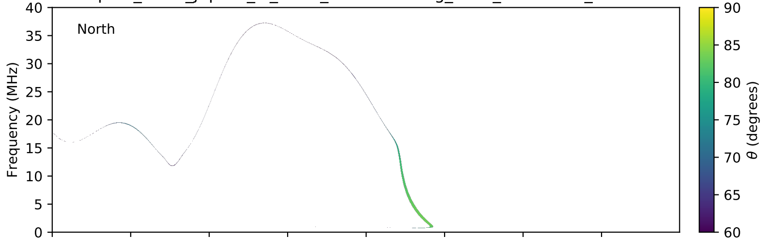
expres_earth_jupiter_io_isaac_lossc-wid1deg_3kev_20151221_v01.cdf
