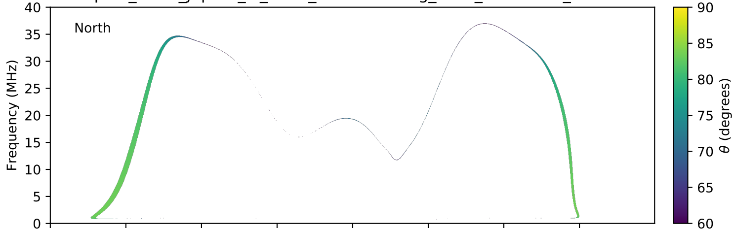
expres_earth_jupiter_io_isaac_lossc-wid1deg_3kev_20151219_v01.cdf
