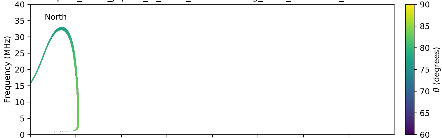
expres_earth_jupiter_io_isaac_lossc-wid1deg_3kev_20151218_v01.cdf
