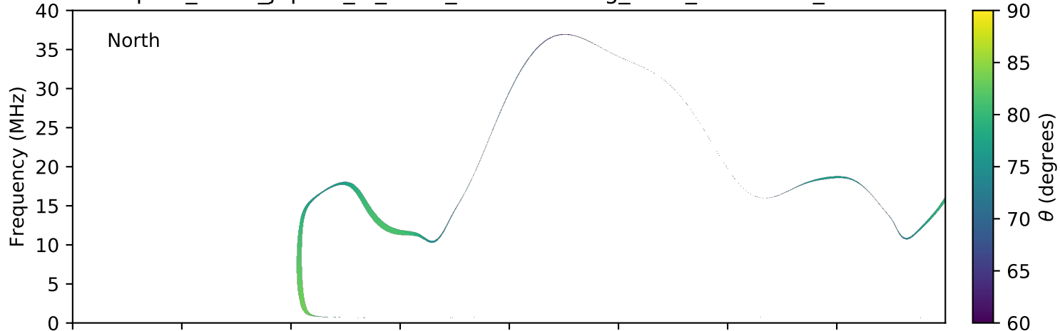
expres_earth_jupiter_io_isaac_lossc-wid1deg_3kev_20151217_v01.cdf
