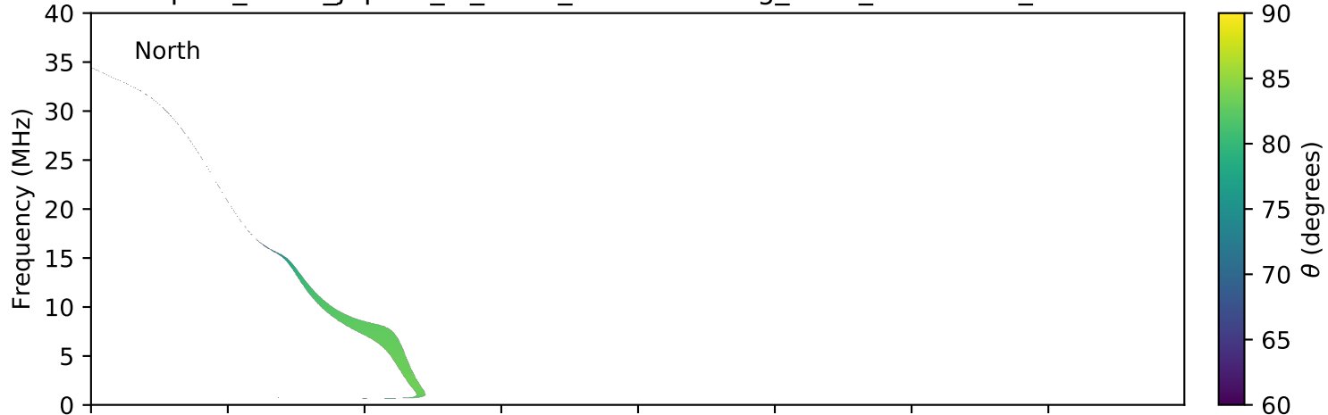
expres_earth_jupiter_io_isaac_lossc-wid1deg_3kev_20151216_v01.cdf
