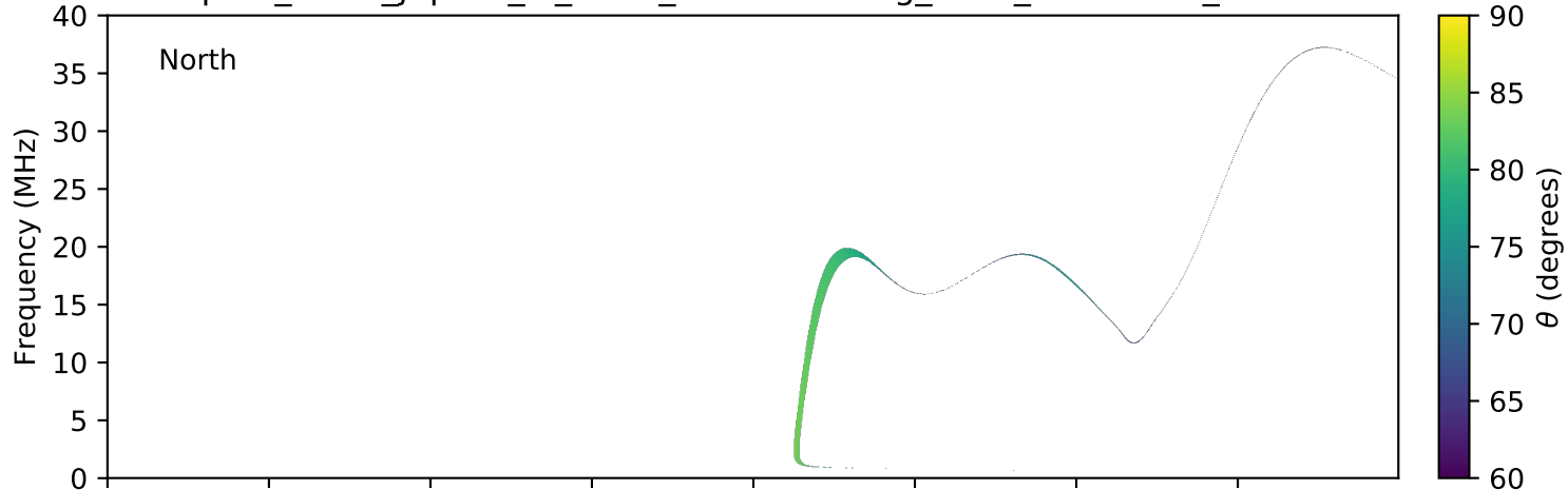
expres_earth_jupiter_io_isaac_lossc-wid1deg_3kev_20151215_v01.cdf
