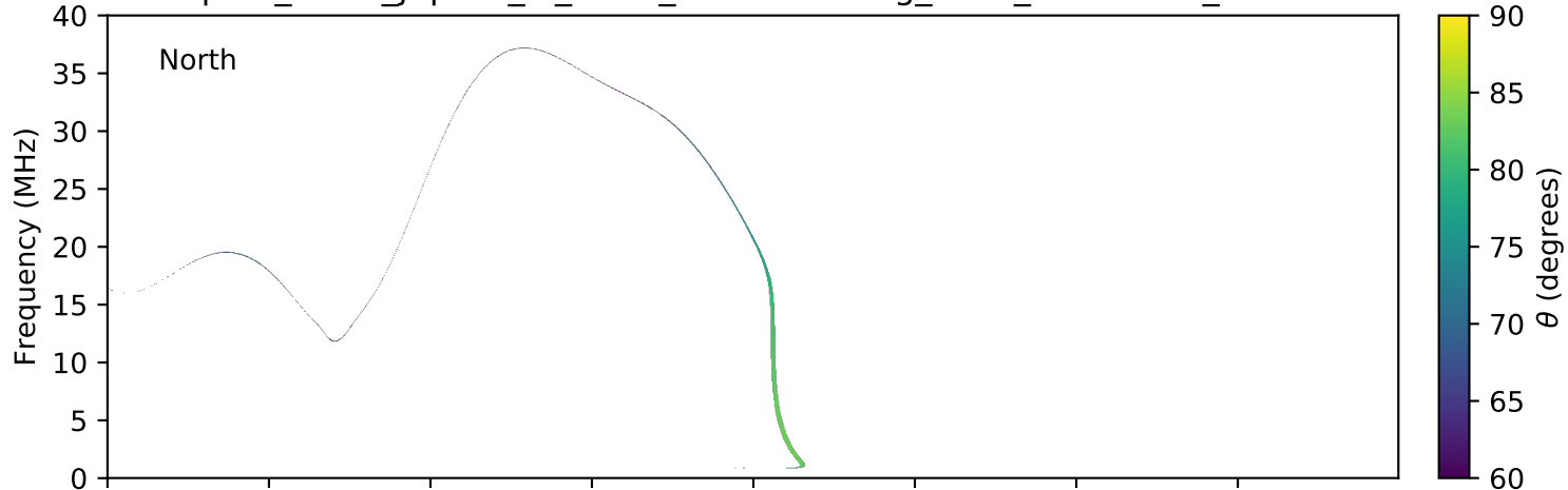
expres_earth_jupiter_io_isaac_lossc-wid1deg_3kev_20151214_v01.cdf
