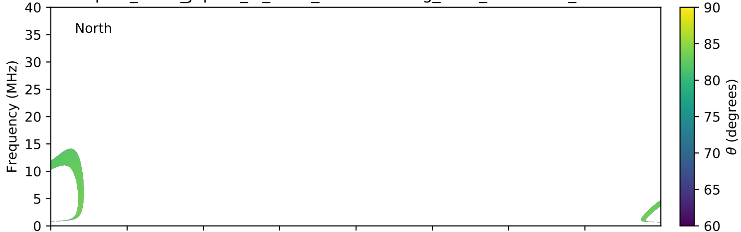
expres_earth_jupiter_io_isaac_lossc-wid1deg_3kev_20151211_v01.cdf
