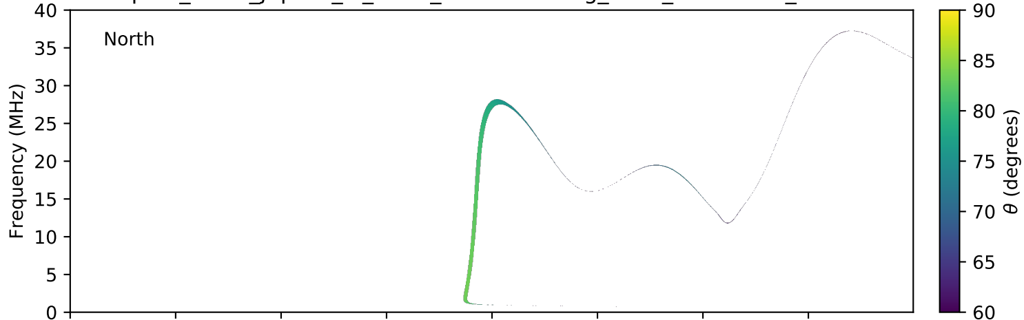
expres_earth_jupiter_io_isaac_lossc-wid1deg_3kev_20151208_v01.cdf
