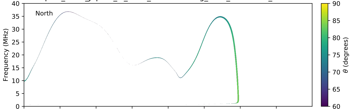
expres_earth_jupiter_io_isaac_lossc-wid1deg_3kev_20151205_v01.cdf
