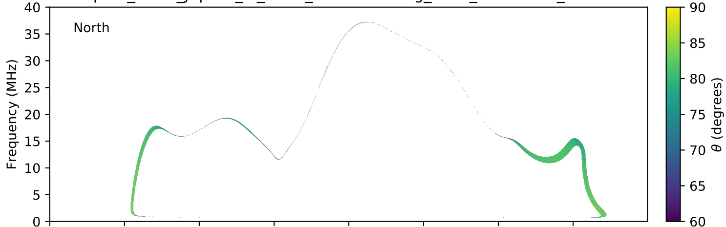
expres_earth_jupiter_io_isaac_lossc-wid1deg_3kev_20151203_v01.cdf
