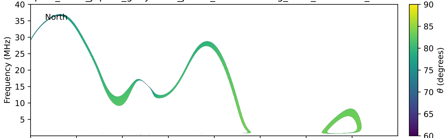
expres_earth_jupiter_ganymede_jrm33_lossc-wid1deg_3kev_20151223_v11.cdf
