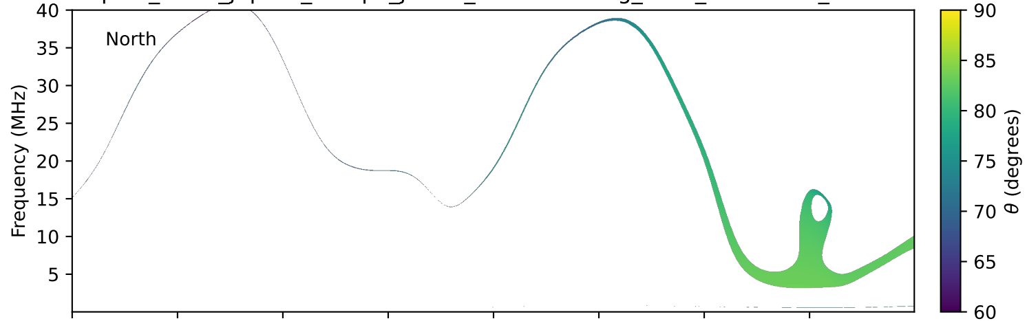
expres_earth_jupiter_europa_jrm33_lossc-wid1deg_3kev_20151203_v11.cdf
