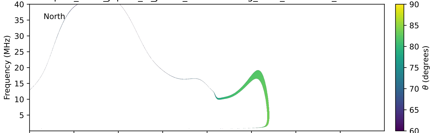
expres_earth_jupiter_io_jrm33_lossc-wid1deg_3kev_20151128_v11.cdf
