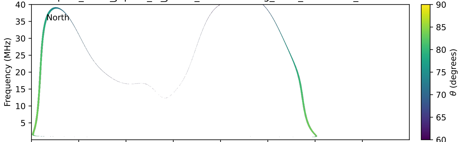
expres_earth_jupiter_io_jrm33_lossc-wid1deg_3kev_20151119_v11.cdf
