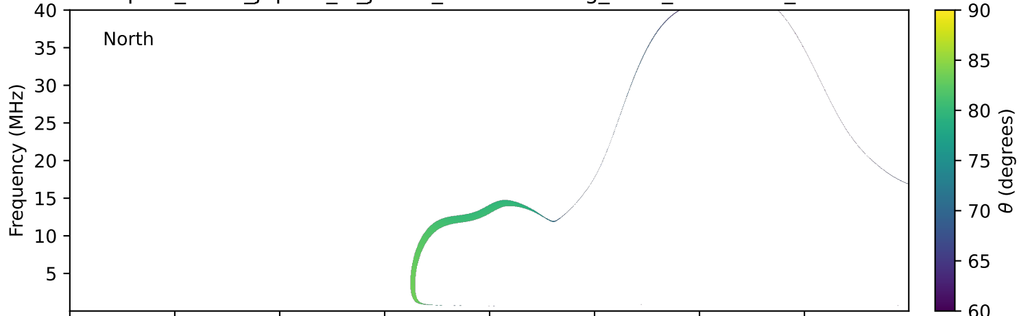
expres_earth_jupiter_io_jrm33_lossc-wid1deg_3kev_20151115_v11.cdf
