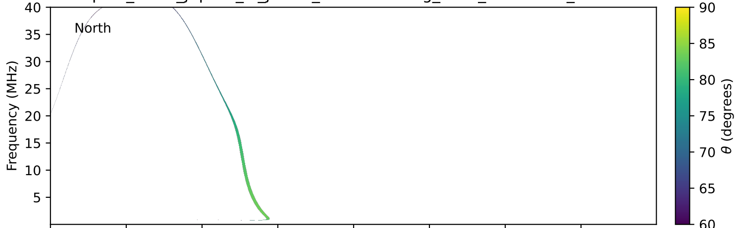
expres_earth_jupiter_io_jrm33_lossc-wid1deg_3kev_20151107_v11.cdf
