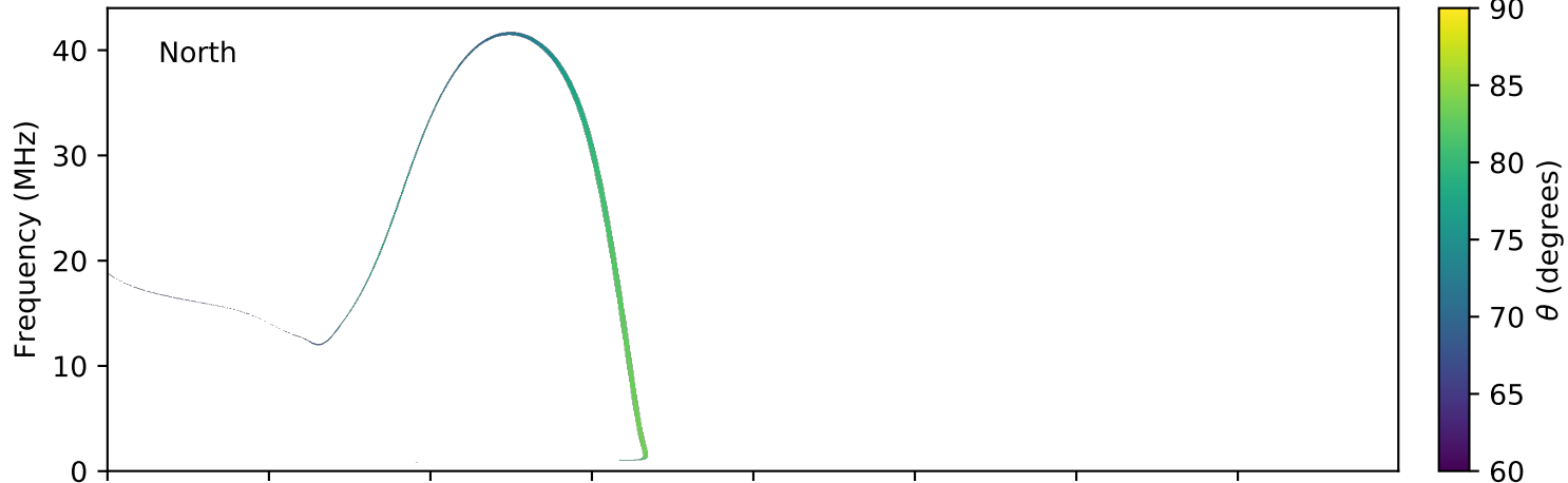
expres_earth_jupiter_io_jrm09_lossc-wid1deg_3kev_20151130_v01.cdf
