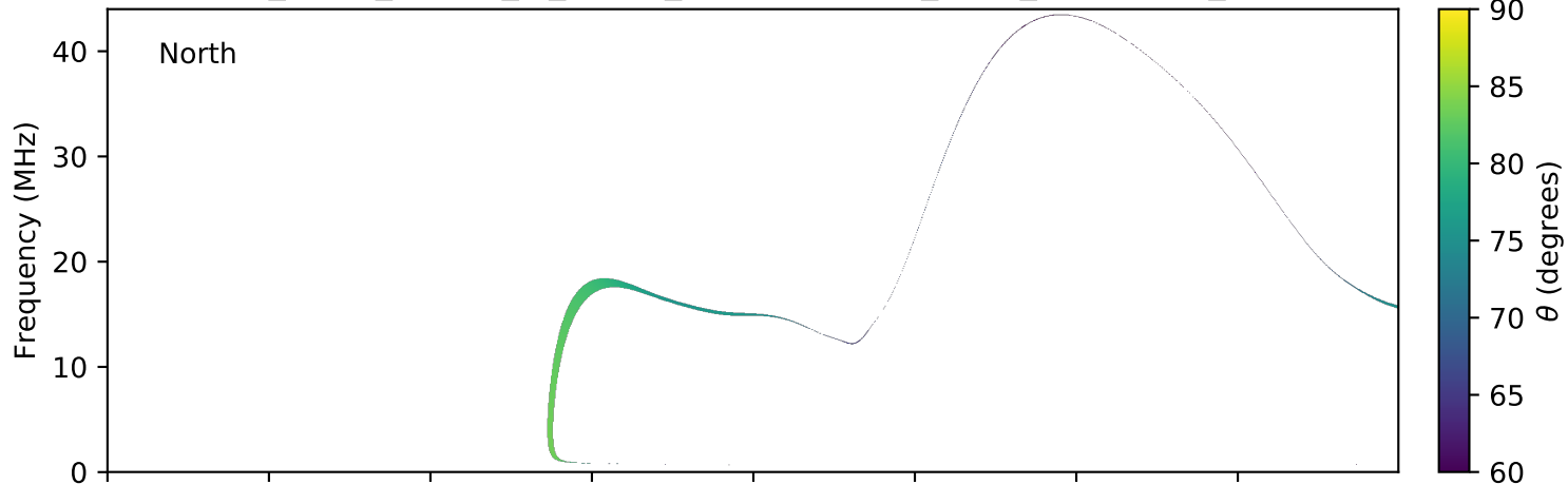
expres_earth_jupiter_io_jrm09_lossc-wid1deg_3kev_20151108_v01.cdf
