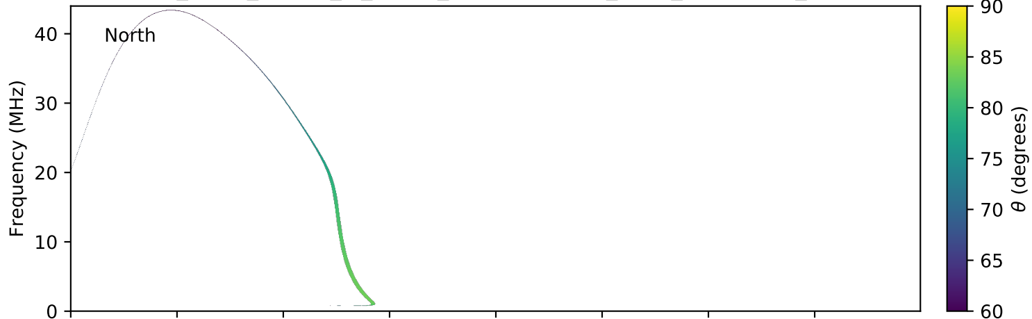
expres_earth_jupiter_io_jrm09_lossc-wid1deg_3kev_20151107_v01.cdf
