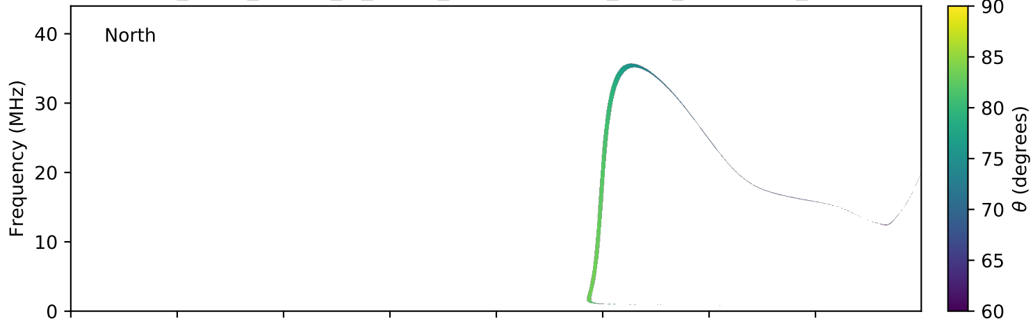
expres_earth_jupiter_io_jrm09_lossc-wid1deg_3kev_20151106_v01.cdf
