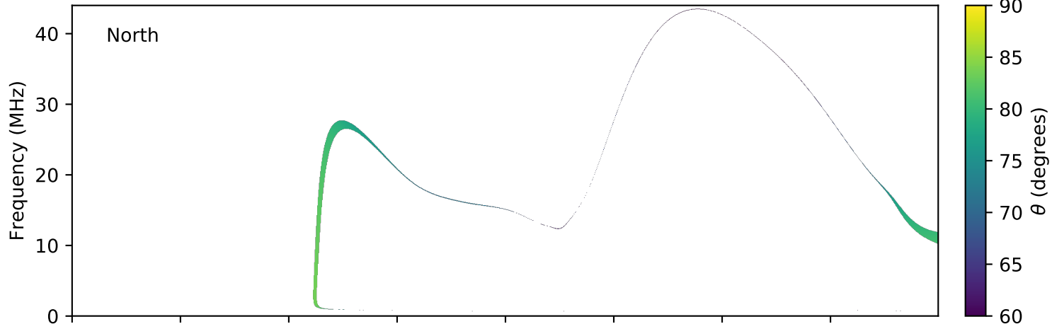
expres_earth_jupiter_io_jrm09_lossc-wid1deg_3kev_20151101_v01.cdf
