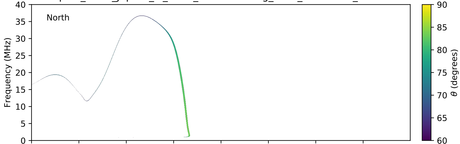
expres_earth_jupiter_io_isaac_lossc-wid1deg_3kev_20151130_v01.cdf
