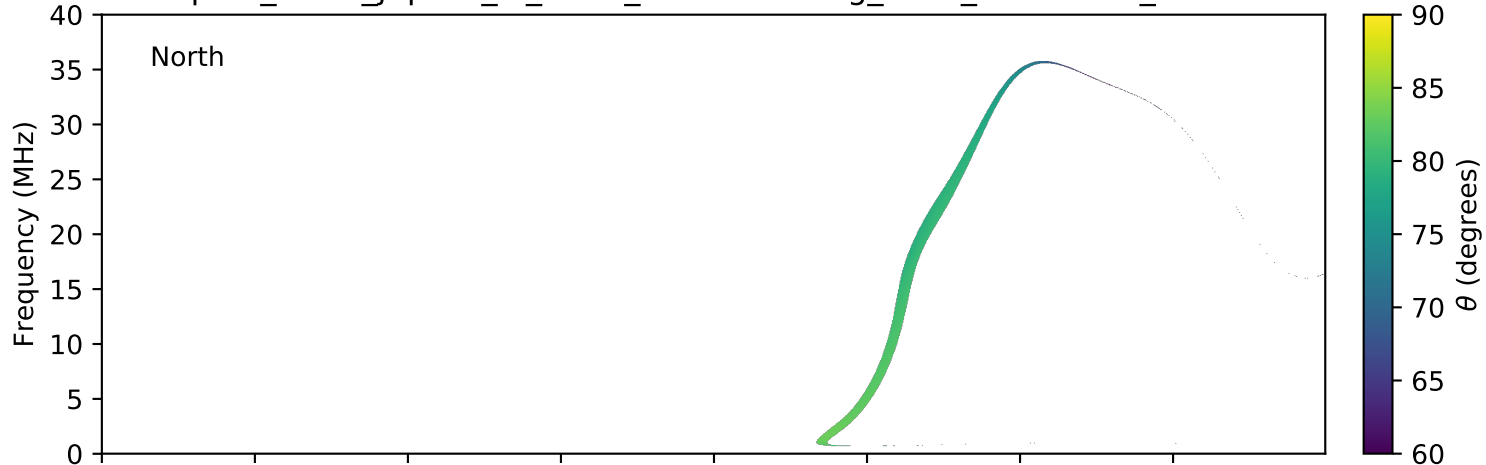
expres_earth_jupiter_io_isaac_lossc-wid1deg_3kev_20151129_v01.cdf
