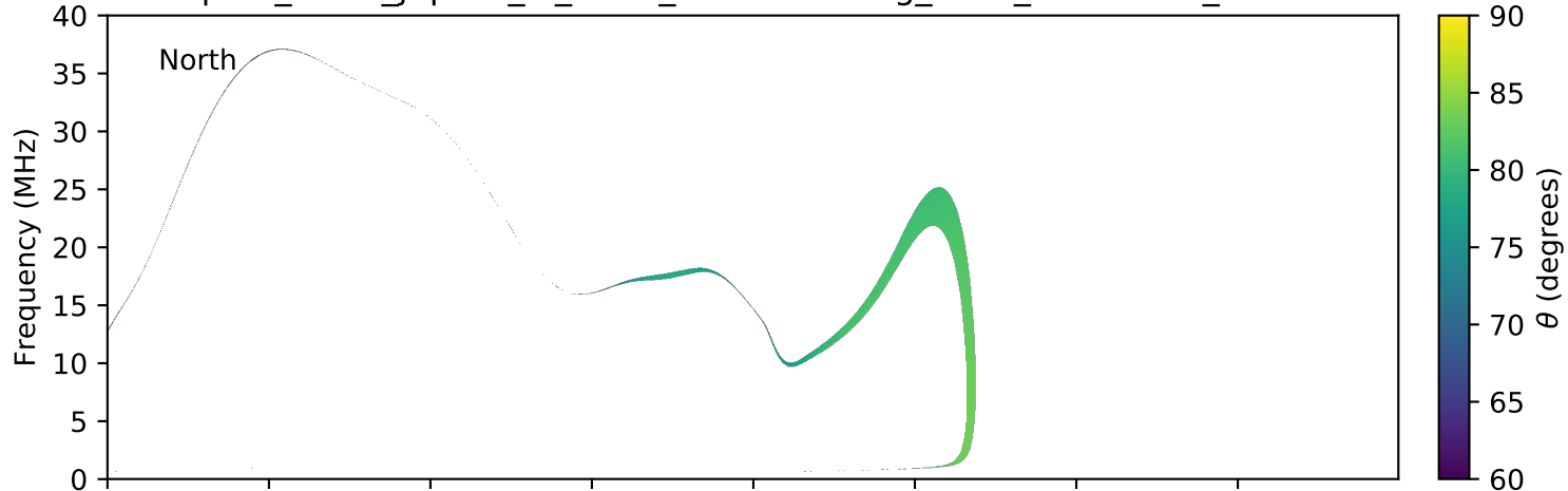
expres_earth_jupiter_io_isaac_lossc-wid1deg_3kev_20151128_v01.cdf
