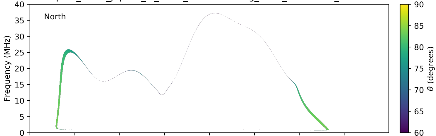
expres_earth_jupiter_io_isaac_lossc-wid1deg_3kev_20151126_v01.cdf
