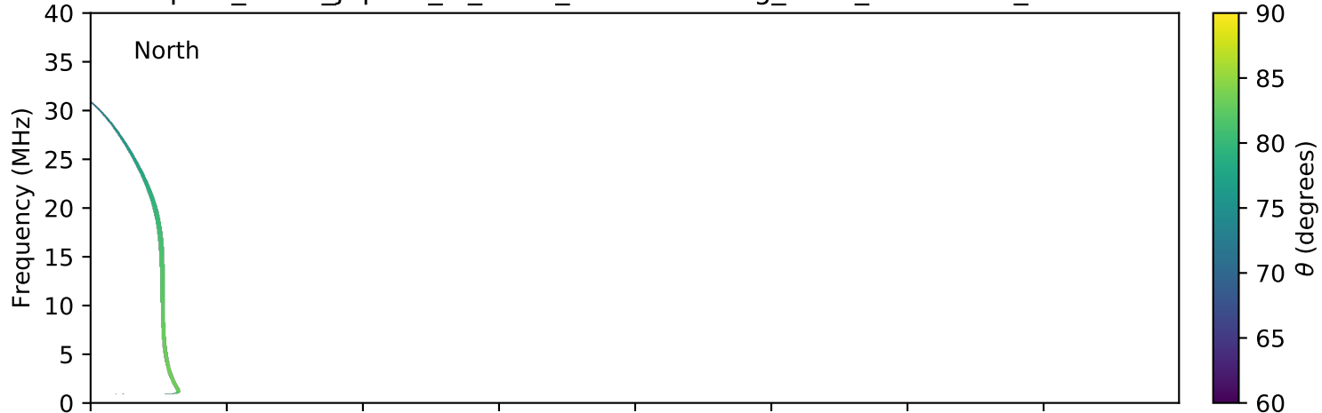
expres_earth_jupiter_io_isaac_lossc-wid1deg_3kev_20151125_v01.cdf
