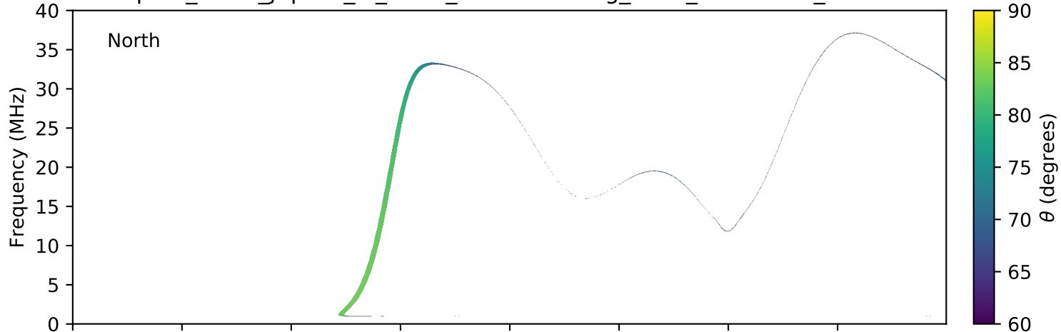
expres_earth_jupiter_io_isaac_lossc-wid1deg_3kev_20151124_v01.cdf
