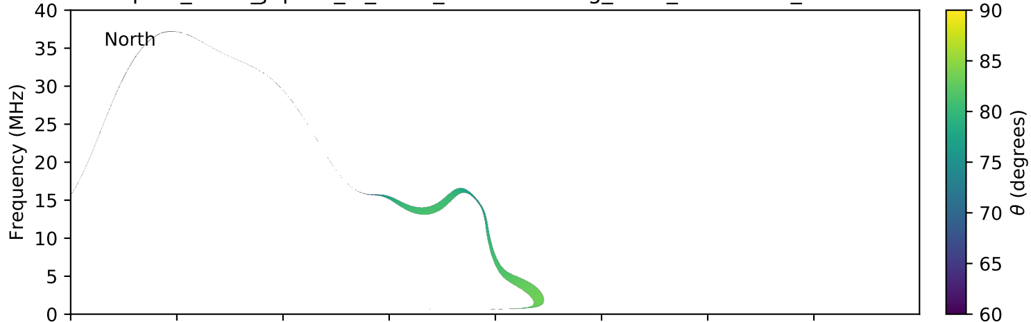
expres_earth_jupiter_io_isaac_lossc-wid1deg_3kev_20151121_v01.cdf
