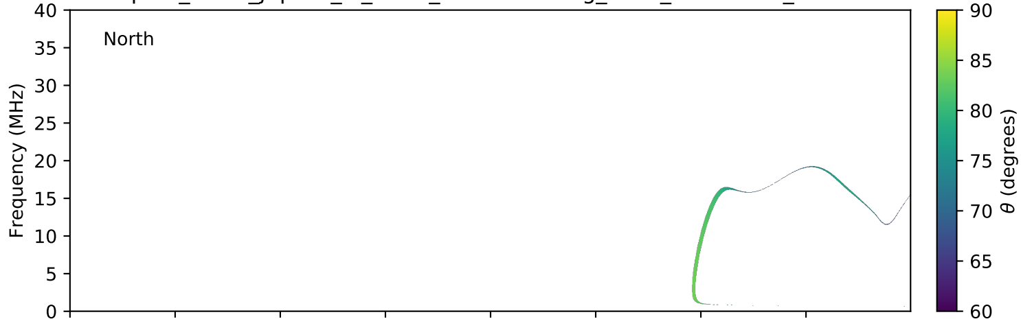
expres_earth_jupiter_io_isaac_lossc-wid1deg_3kev_20151120_v01.cdf
