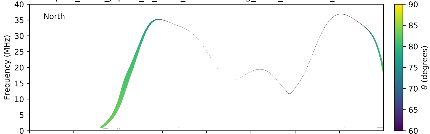
expres_earth_jupiter_io_isaac_lossc-wid1deg_3kev_20151117_v01.cdf
