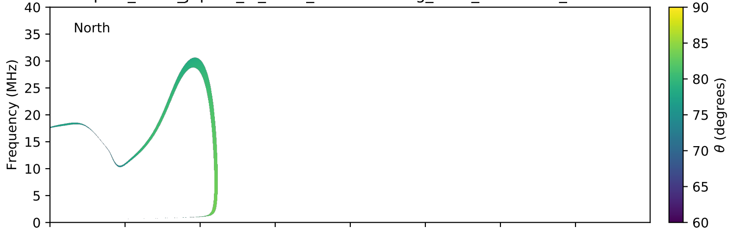
expres_earth_jupiter_io_isaac_lossc-wid1deg_3kev_20151116_v01.cdf
