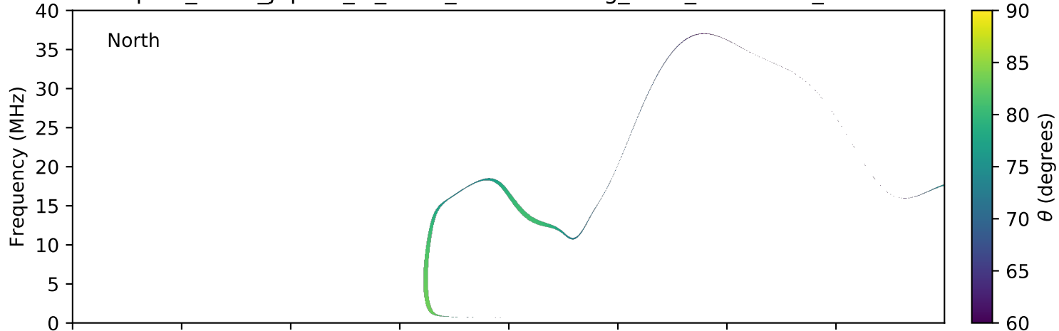
expres_earth_jupiter_io_isaac_lossc-wid1deg_3kev_20151115_v01.cdf
