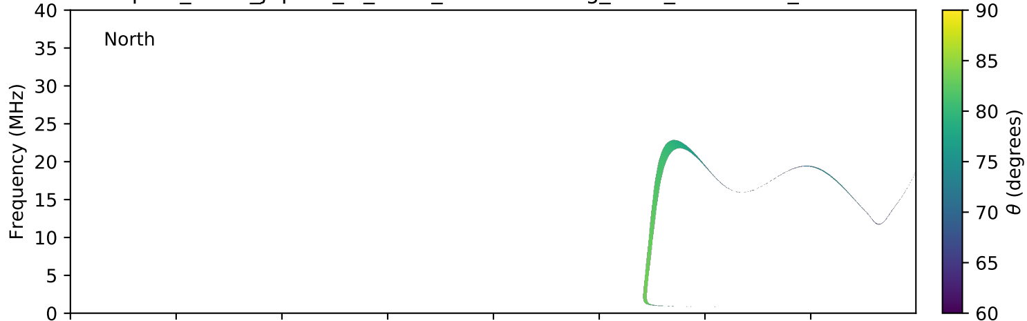
expres_earth_jupiter_io_isaac_lossc-wid1deg_3kev_20151113_v01.cdf
