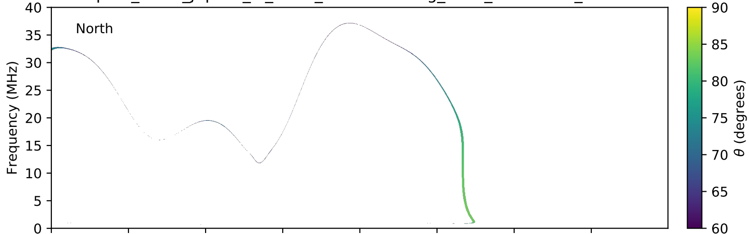
expres_earth_jupiter_io_isaac_lossc-wid1deg_3kev_20151112_v01.cdf
