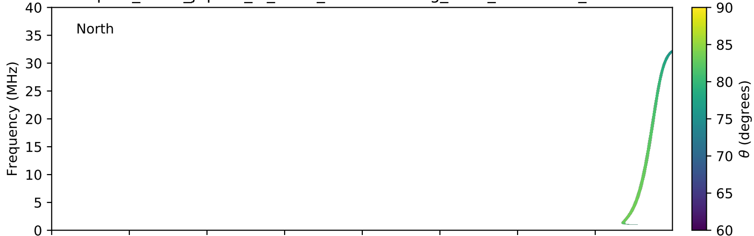
expres_earth_jupiter_io_isaac_lossc-wid1deg_3kev_20151111_v01.cdf
